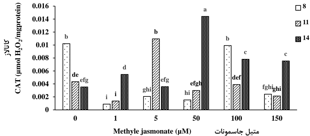
Fig. 10. The effect of methyl jasmonate on CAT enzyme of cucurbita pepo under chilling stress. Means followed by the same letters are not significantly different (LSD 0.05 ).
