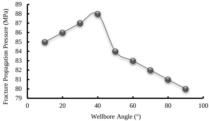
Fig. 9. Minimum fracture propagation pressure versus wellbore angle
