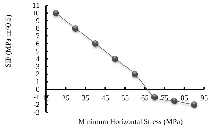
Fig. 4. Variations of minimum horizontal stress relative to the SIF
