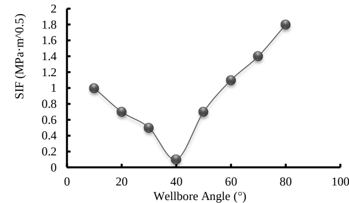
Fig. 8. Variations of the wellbore angle as a function of the SIF
