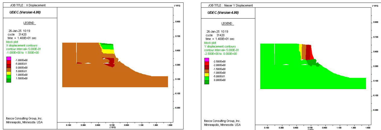
Fig. 15. The X and Y displacement model indicates that the combined presence of cracks, voids, and the vertical load of the Niasar building caused displacement, which moved the block from the tip and pushed the slope toward failure.
