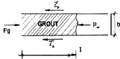
Fig. 2. Grout penetration into a fracture
