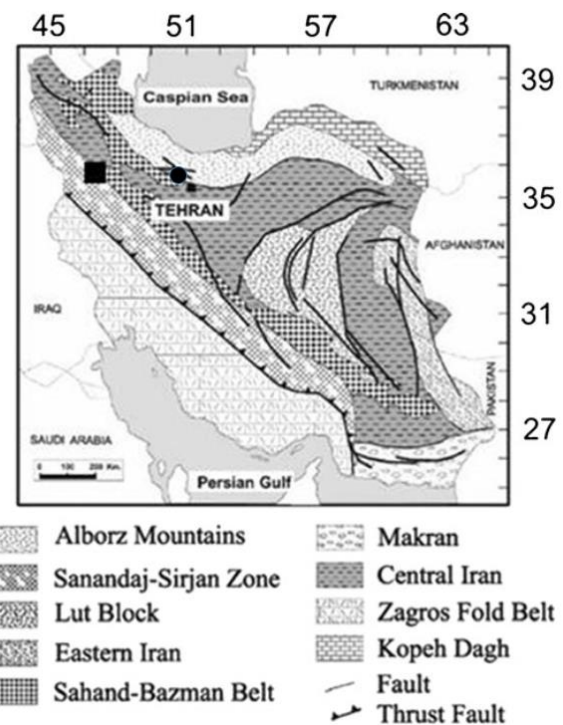
Fig. 4. Azad powerplant(black square) and Siahbishe powerplant(black circle) on Iran geological map
