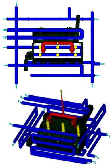
Fig. 4. Designed cooling system (2) in two views.
