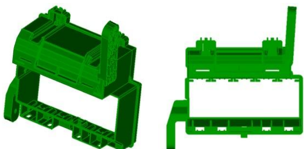
Fig. 1. 3D model of Peugeot 206 engine compartment fuse/relay frame part.
