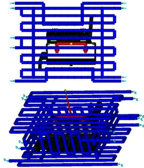
Fig. 5. Designed cooling system (3) in two views.
