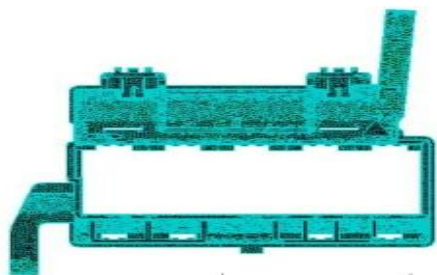
Fig. 2. Meshed model of the part.
