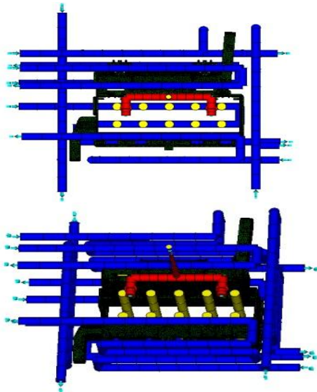
Fig. 3. Designed cooling system (1) in two views.
