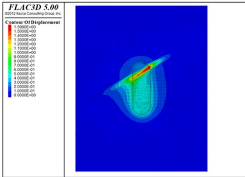
Fig. 7. Total displacement of geo6 model at the end of operational time
