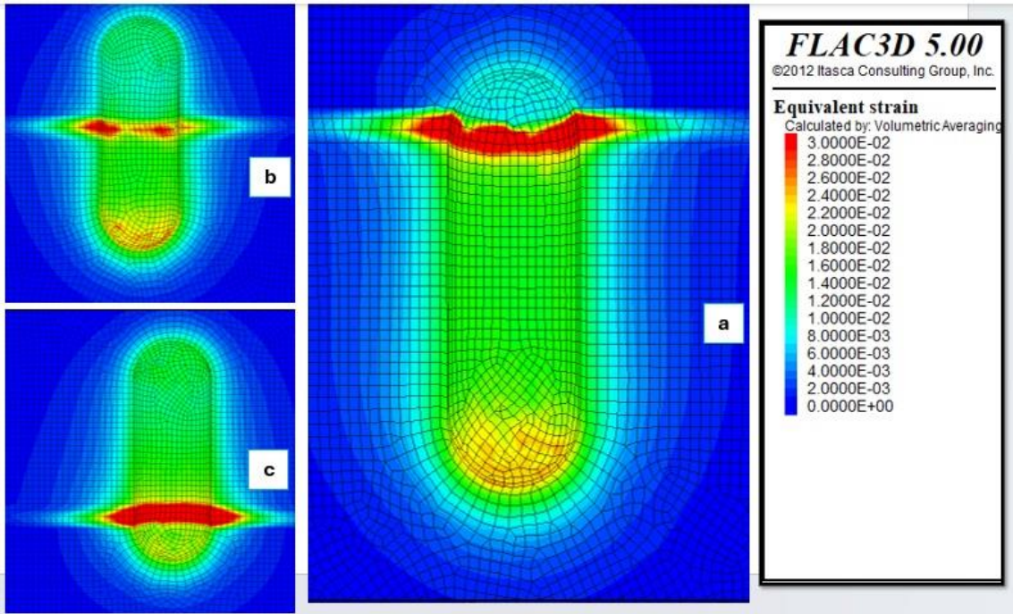
Fig. 14. Equivalent strain contour around the salt cavern: a) Interlayer at level A, b) Interlayer at level B, and c) Interlayer at level C
