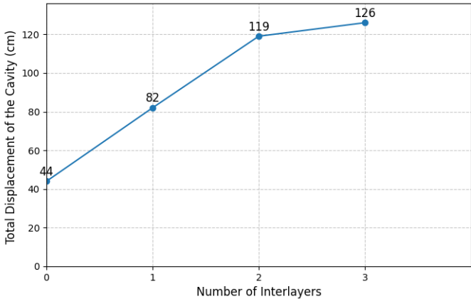
Fig. 13. Effect of interlayers numbers on total displacement
