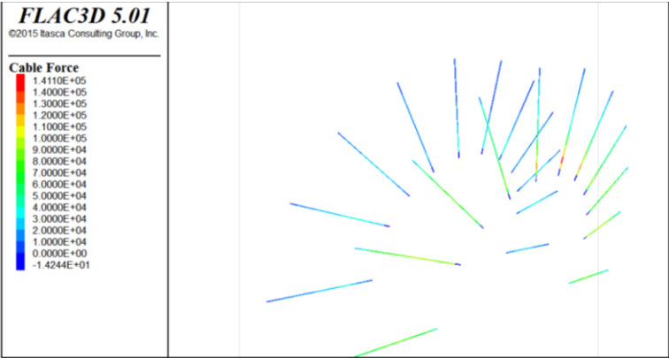
Fig 11. Axial force of bolt in the third excavation step, with shotcrete installation in the first excavation step
