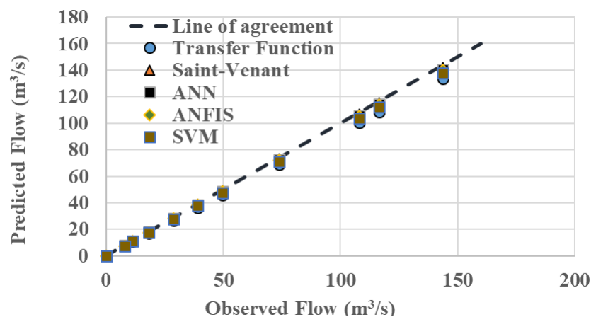
Fig. 9. Observed and Predicted Peak Flows for the 2019 Flood Event ( \text{m}^3/\text{s} )
